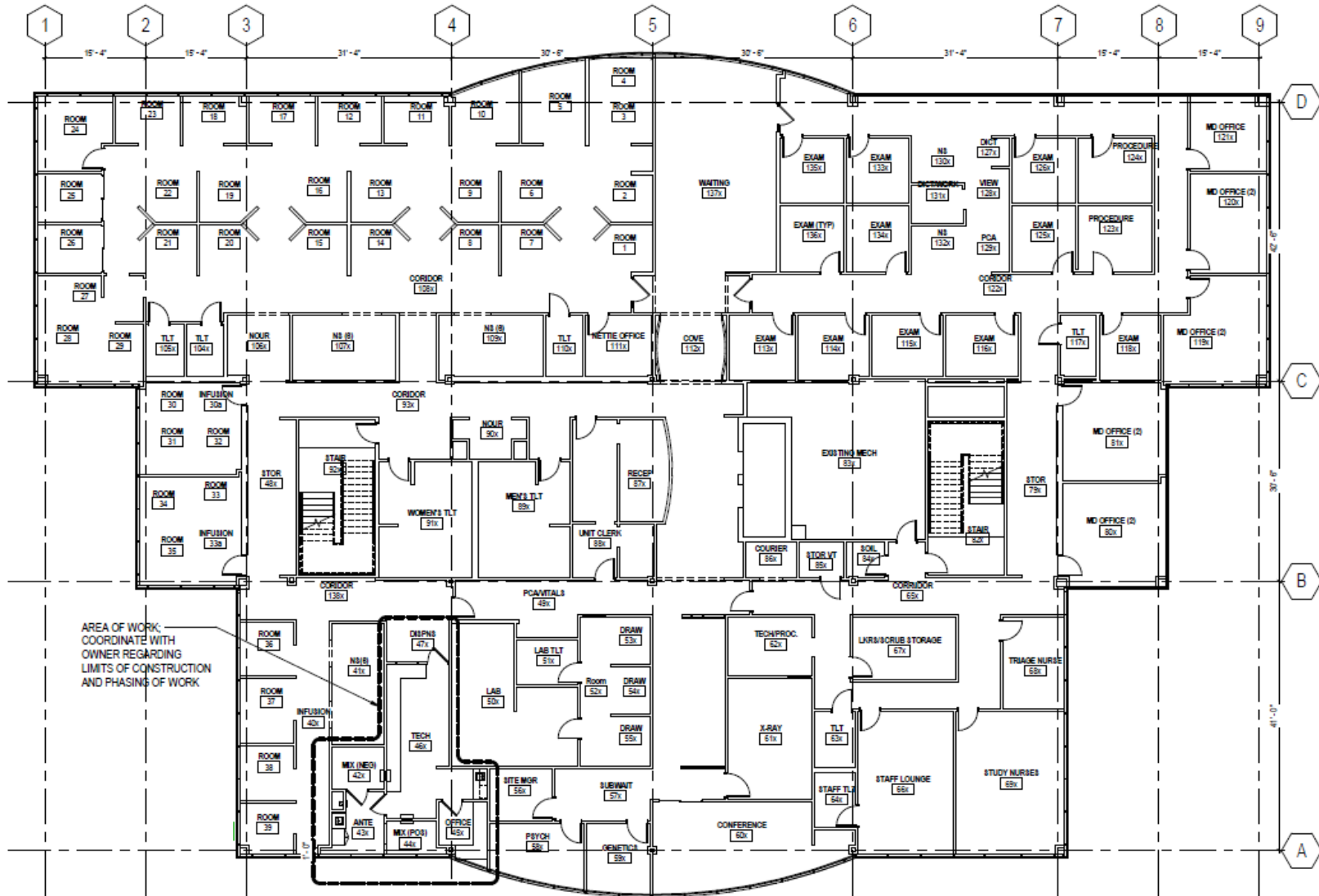
① 04 FOURTH FLOOR PLAN-EXIST 3/32" = 1'-0"
